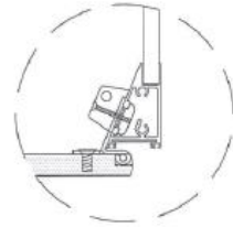
Optional Design Concealed Hinge
