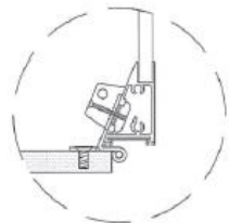
Standard Design Non Concealed Hinge
